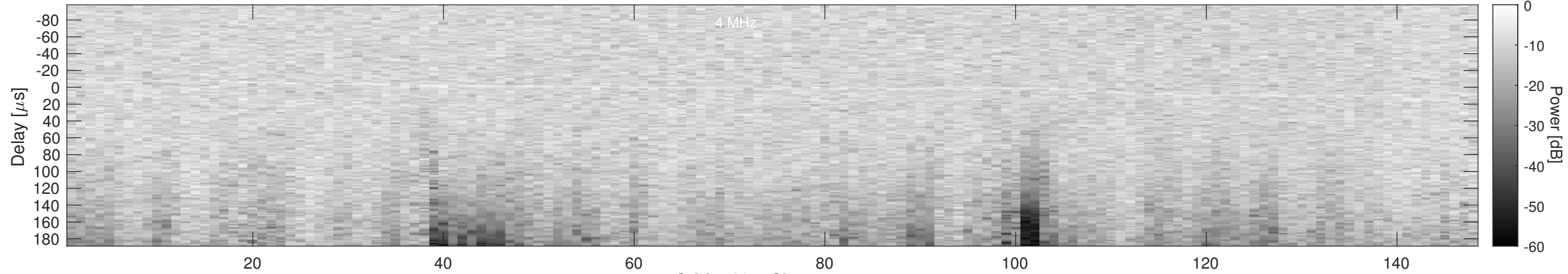
Orbit 4297, Cluttergram
