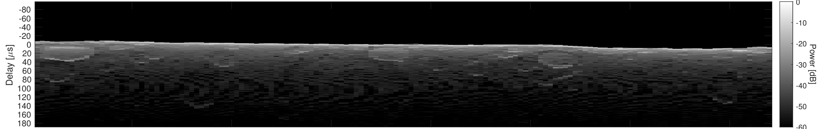
Orbit 4297, Cluttergram
