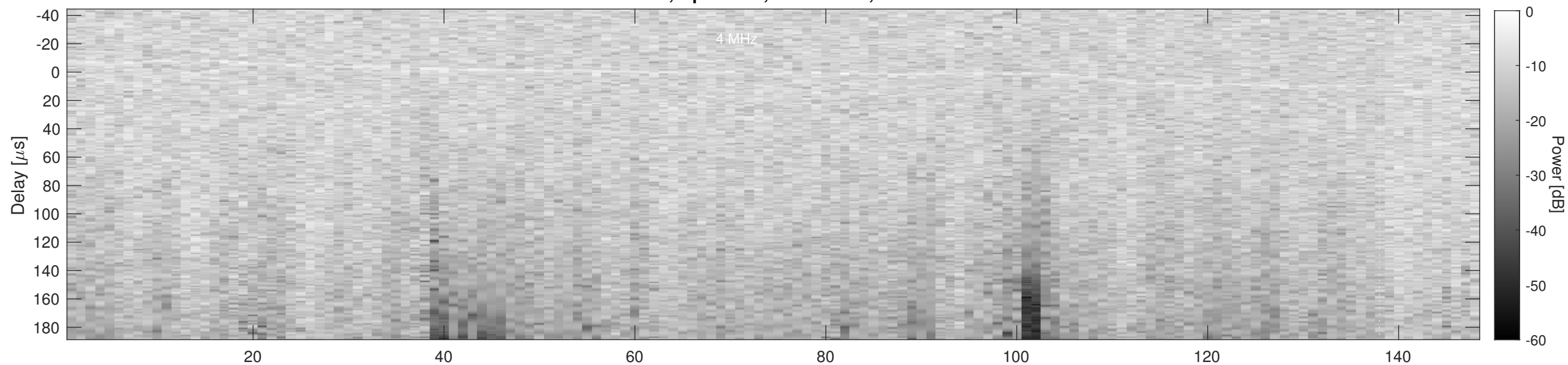
Orbit 4297, Cluttergram
