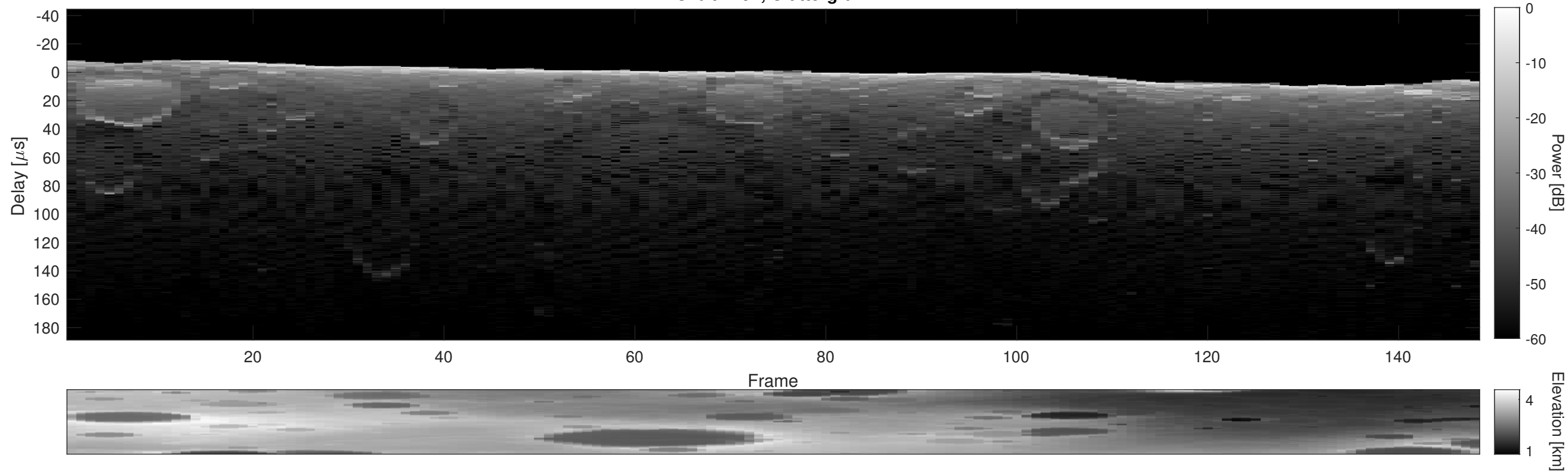
Orbit 4297, Cluttergram
