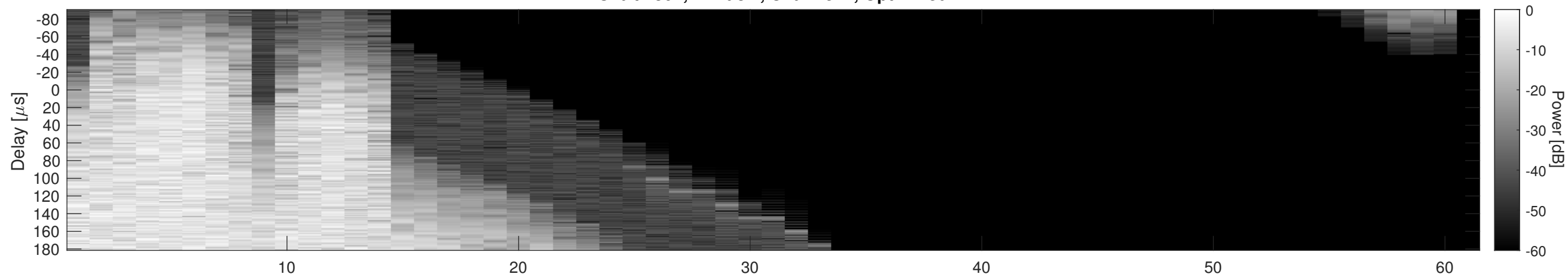
Orbit 4307, Cluttergram
