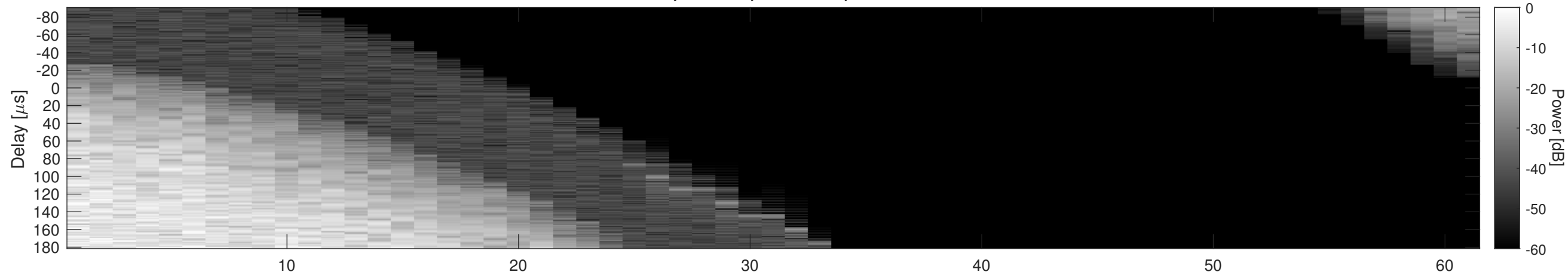
Orbit 4307, Window, Channel 2, Chapman
