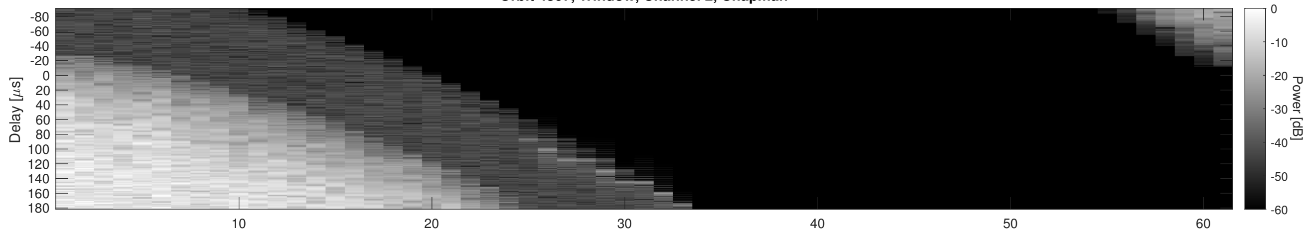
Orbit 4307, Window, Channel 2, Optimized
