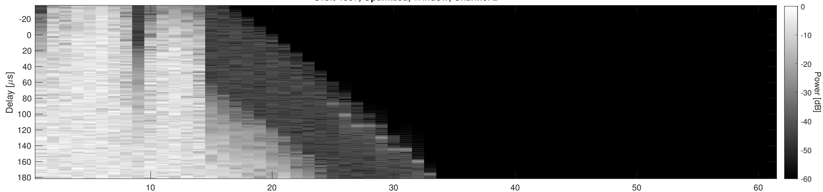
Orbit 4307, Cluttergram
