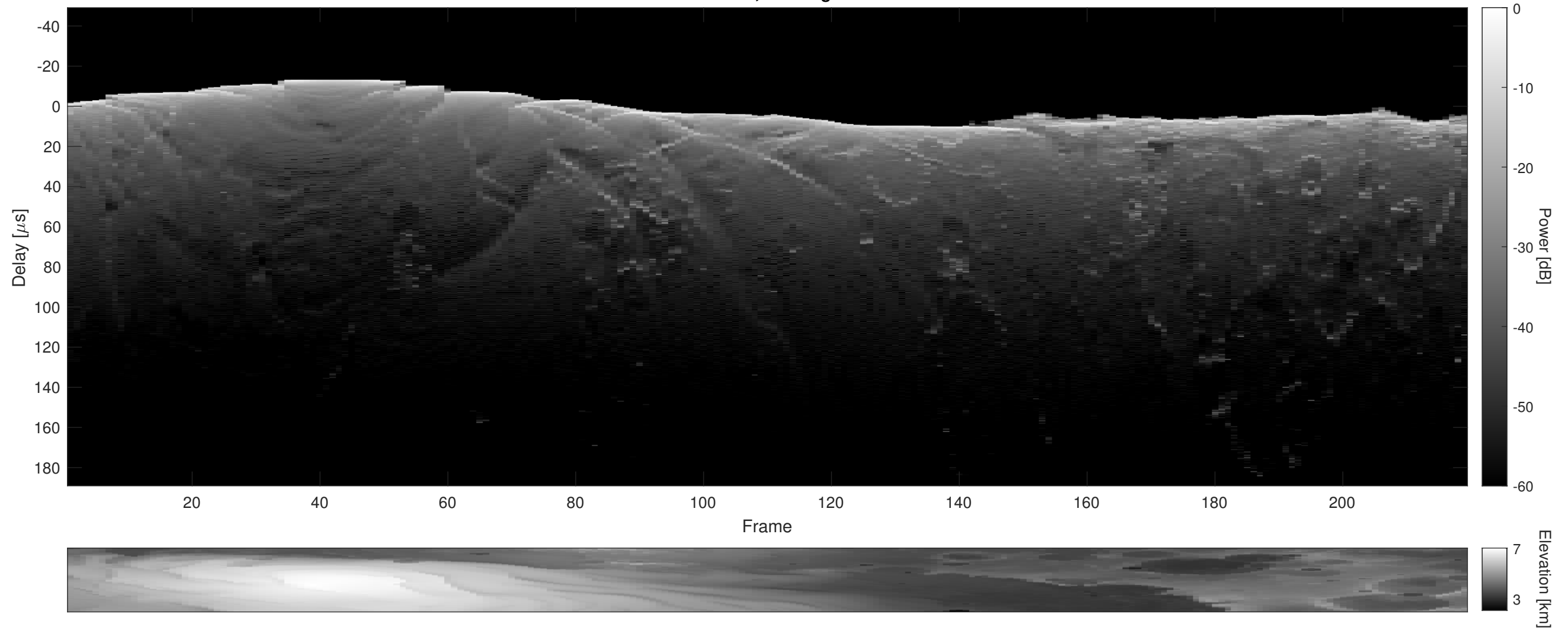
Orbit 4309, Cluttergram
