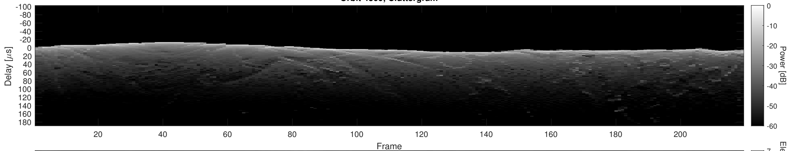
Orbit 4309, Cluttergram
