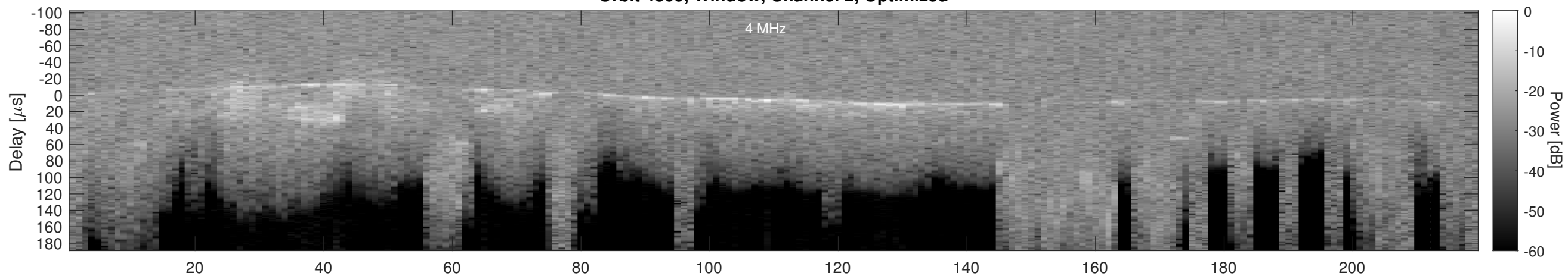
Orbit 4309, Cluttergram
