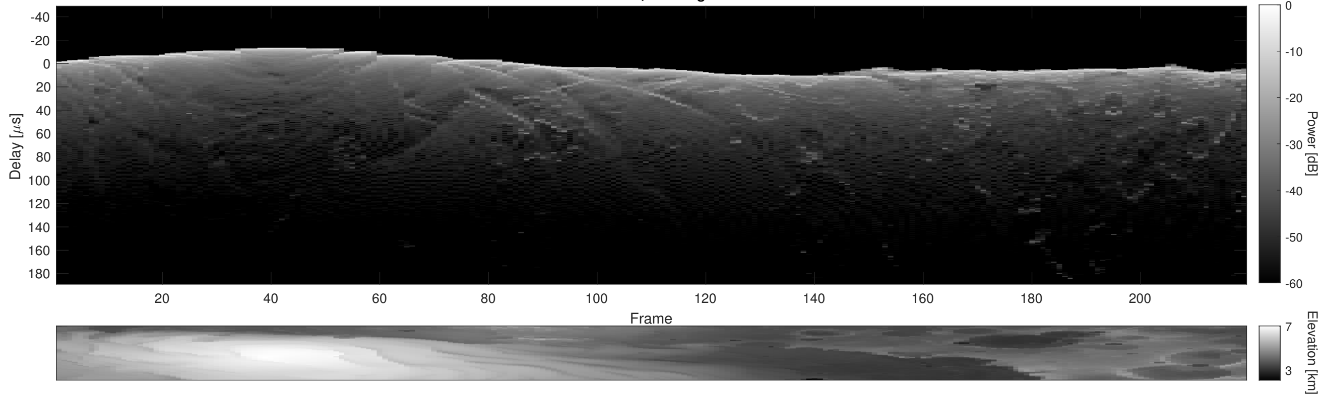
Orbit 4309, Cluttergram
