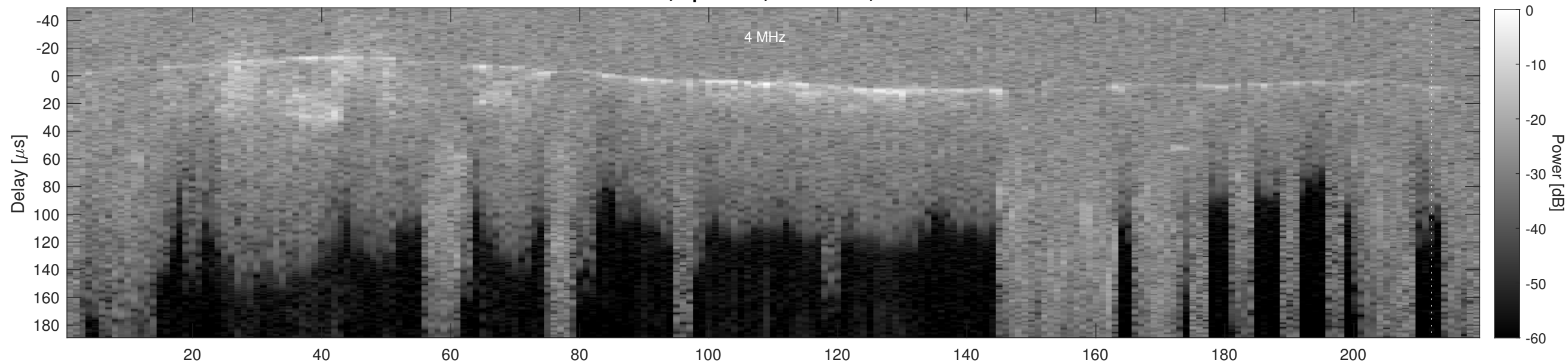
Orbit 4309, Cluttergram
