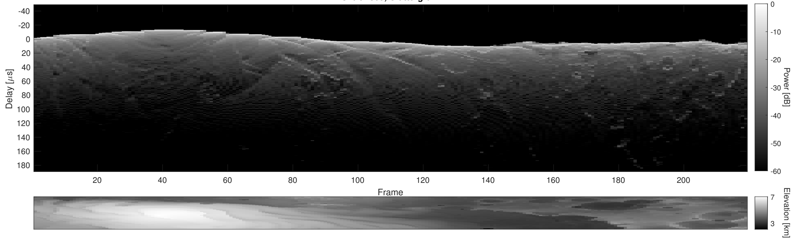
Orbit 4309, Cluttergram
