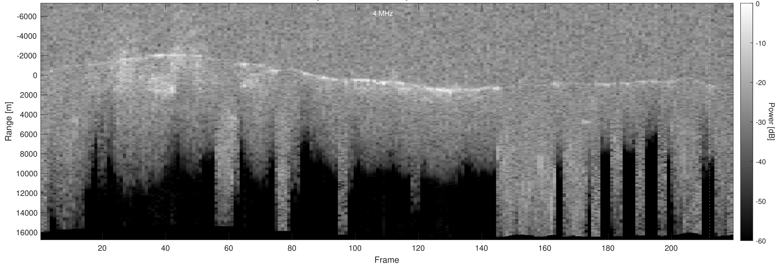
Orbit 4309, Optimized, Window, Depth-Corrected, Channel 2
