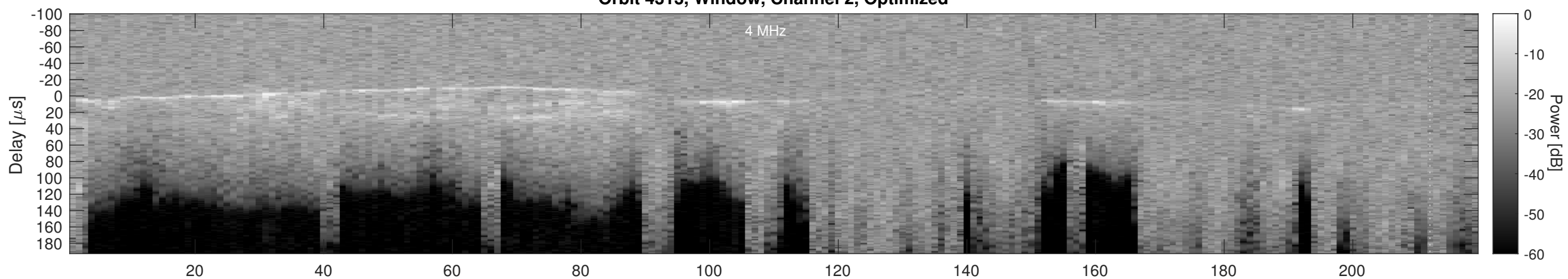
Orbit 4313, Cluttergram
