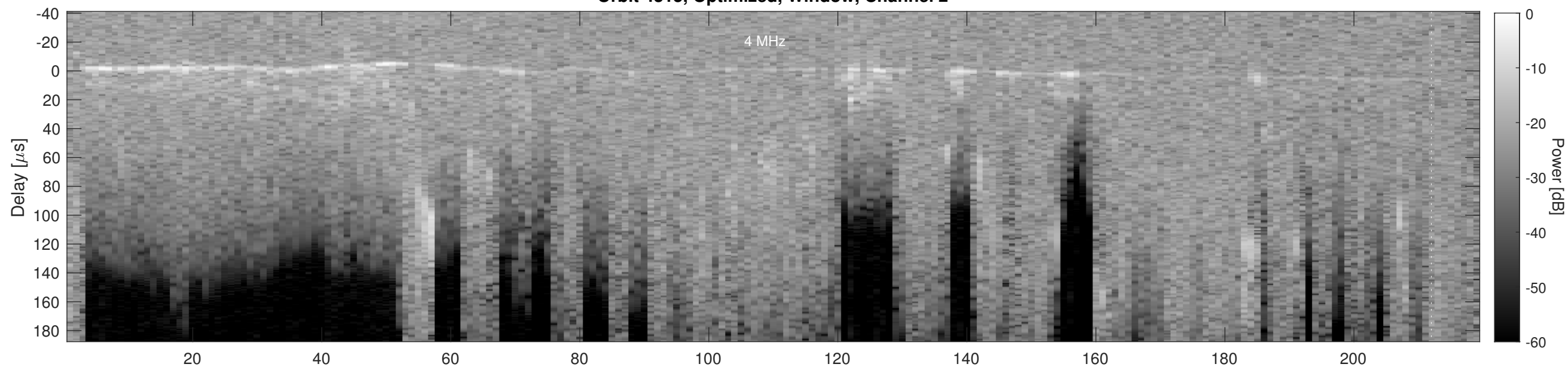
Orbit 4315, Cluttergram
