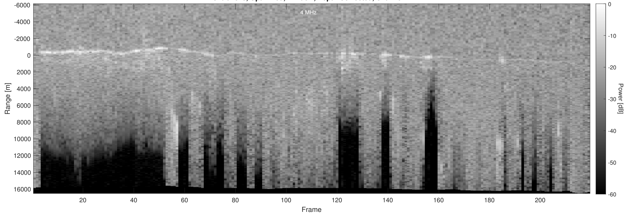
Orbit 4315, Optimized, Window, Depth-Corrected, Channel 2
