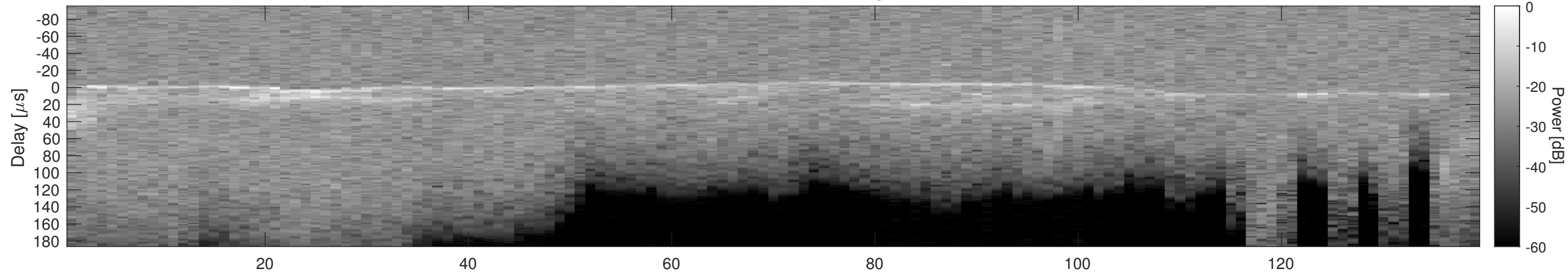
Orbit 4317, Cluttergram
