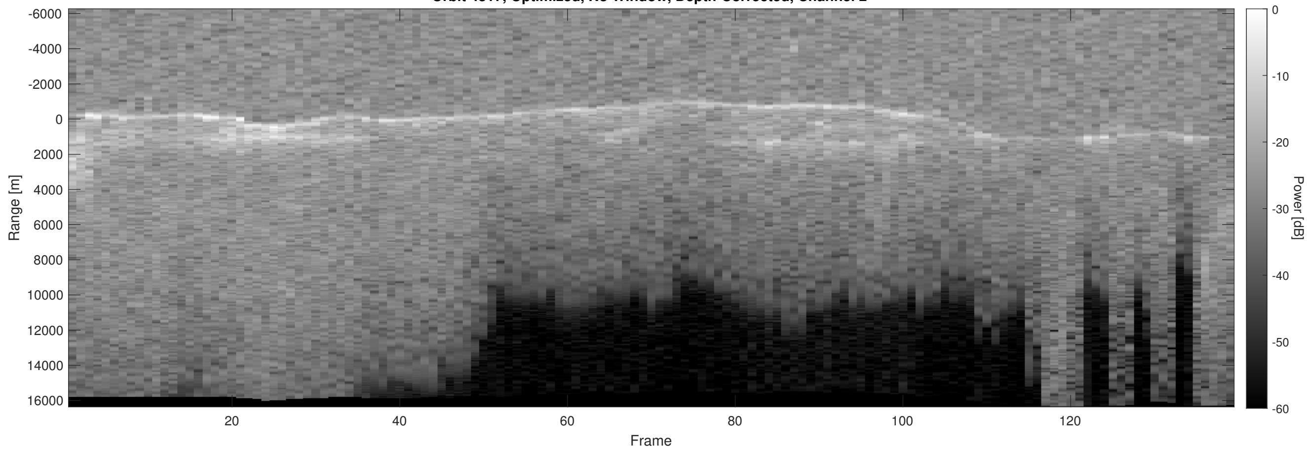
Orbit 4317, Optimized, No Window, Depth-Corrected, Channel 2
