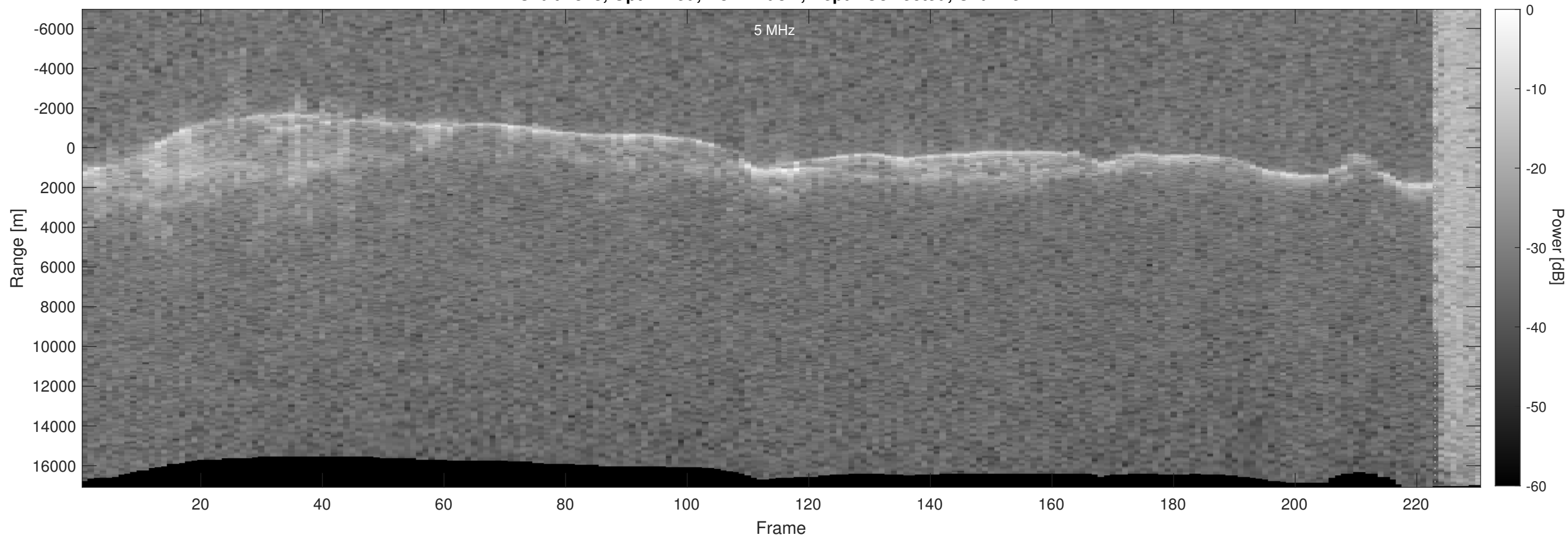
Orbit 4323, Optimized, No Window, Depth-Corrected, Channel 2
