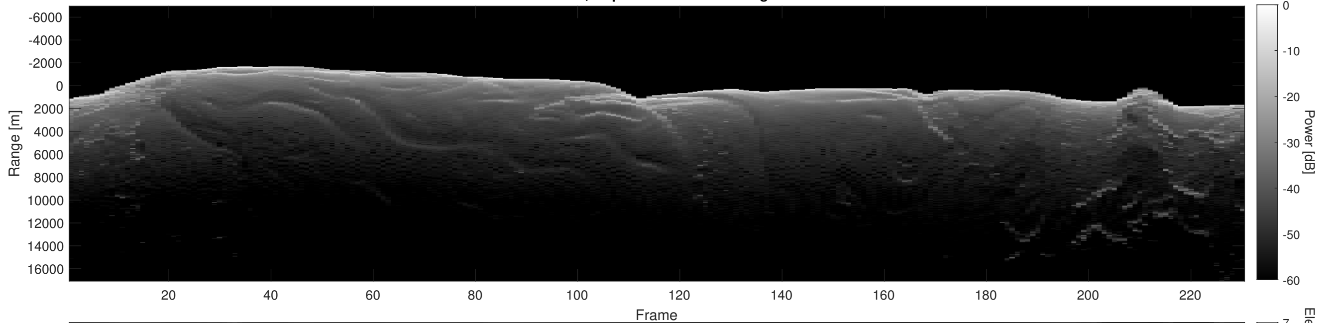
Orbit 4323, Depth-Corrected Cluttergram
