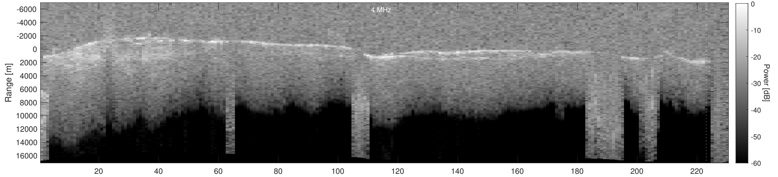
Orbit 4323, Depth-Corrected Cluttergram
