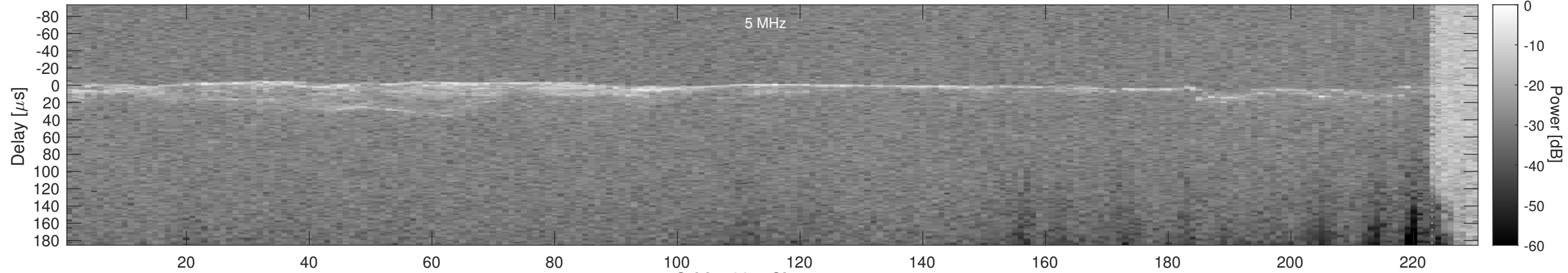
Orbit 4325, Cluttergram
