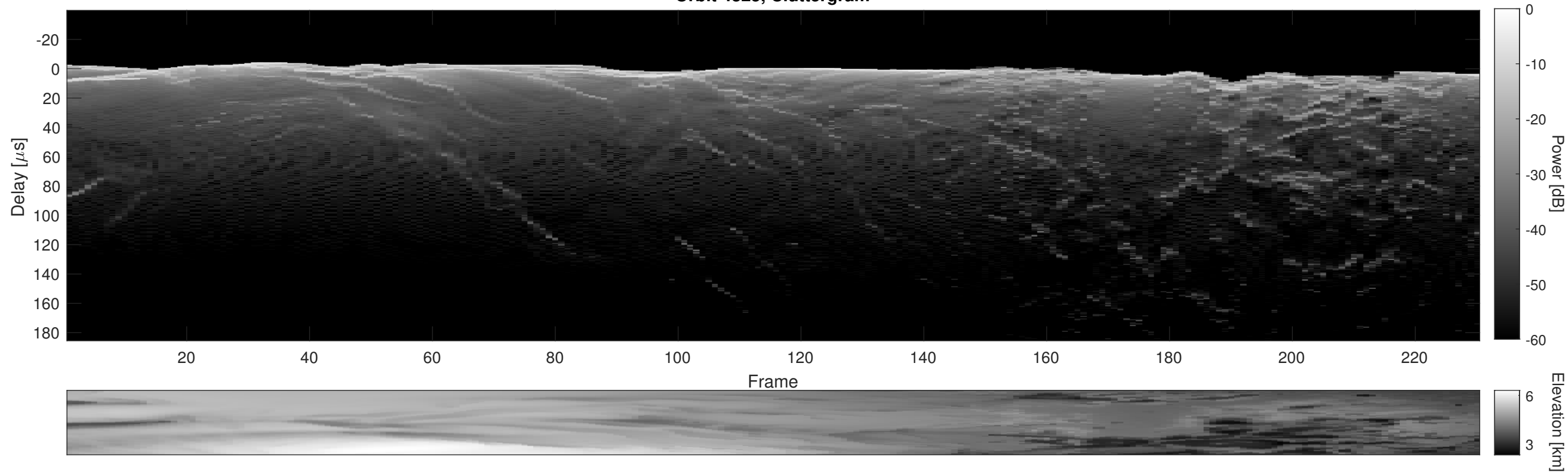
Orbit 4325, Cluttergram
