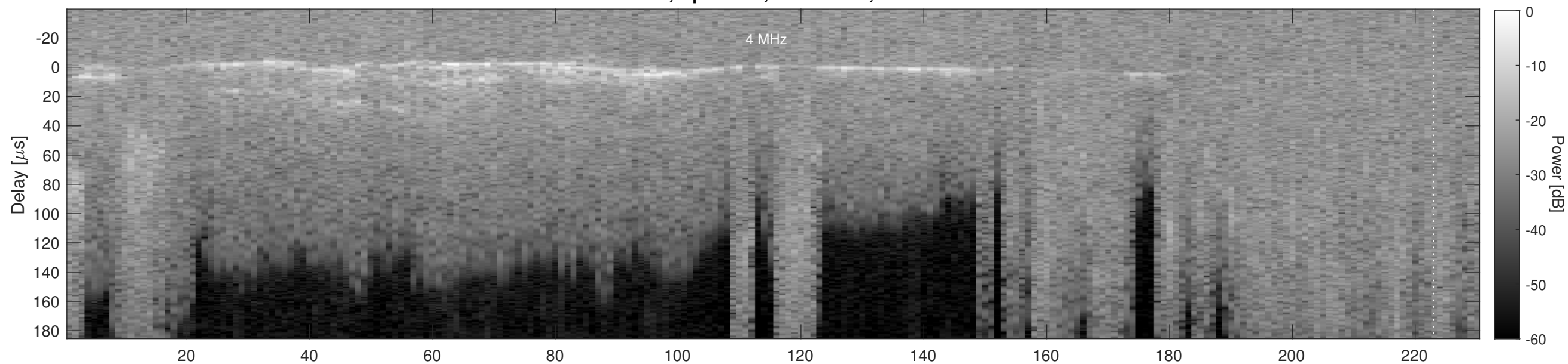
Orbit 4325, Cluttergram
