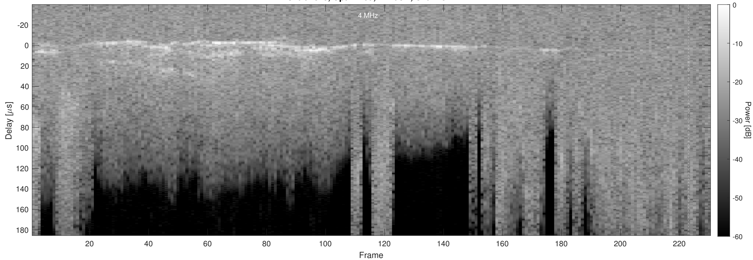
Orbit 4325, Optimized, Window, Channel 2
