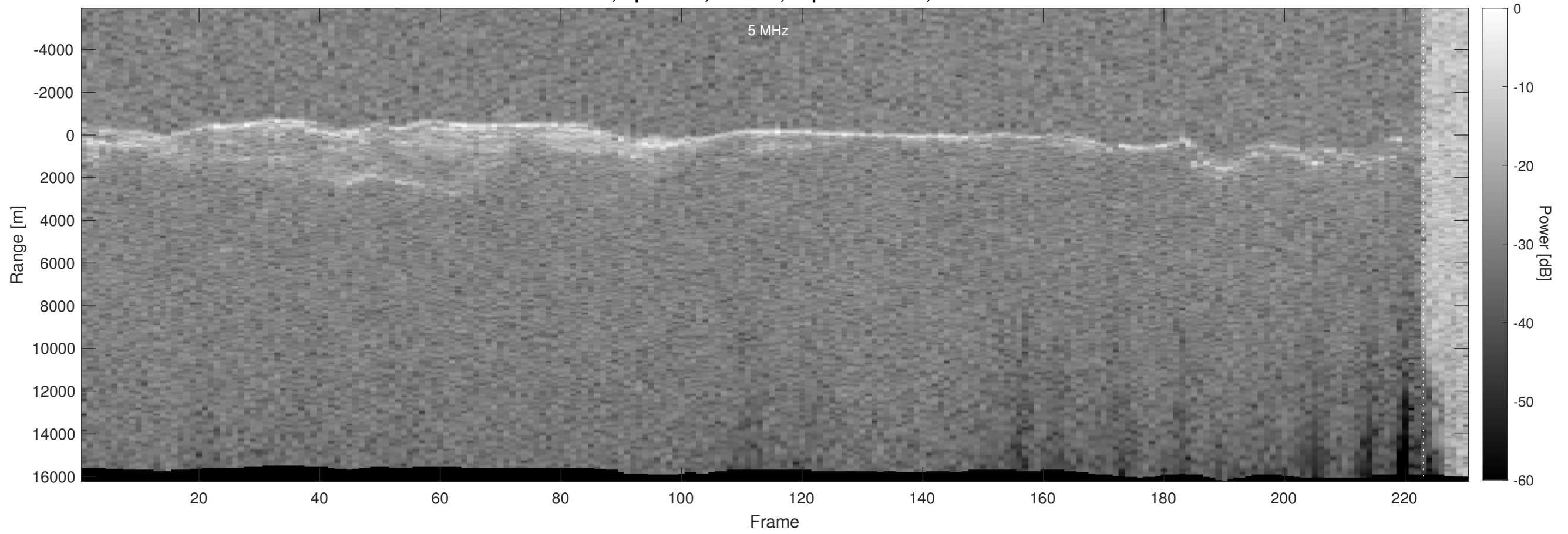
Orbit 4325, Optimized, Window, Depth-Corrected, Channel 2
