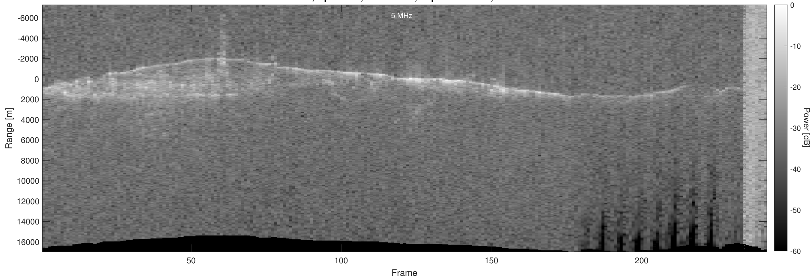
Orbit 4327, Optimized, No Window, Depth-Corrected, Channel 2
