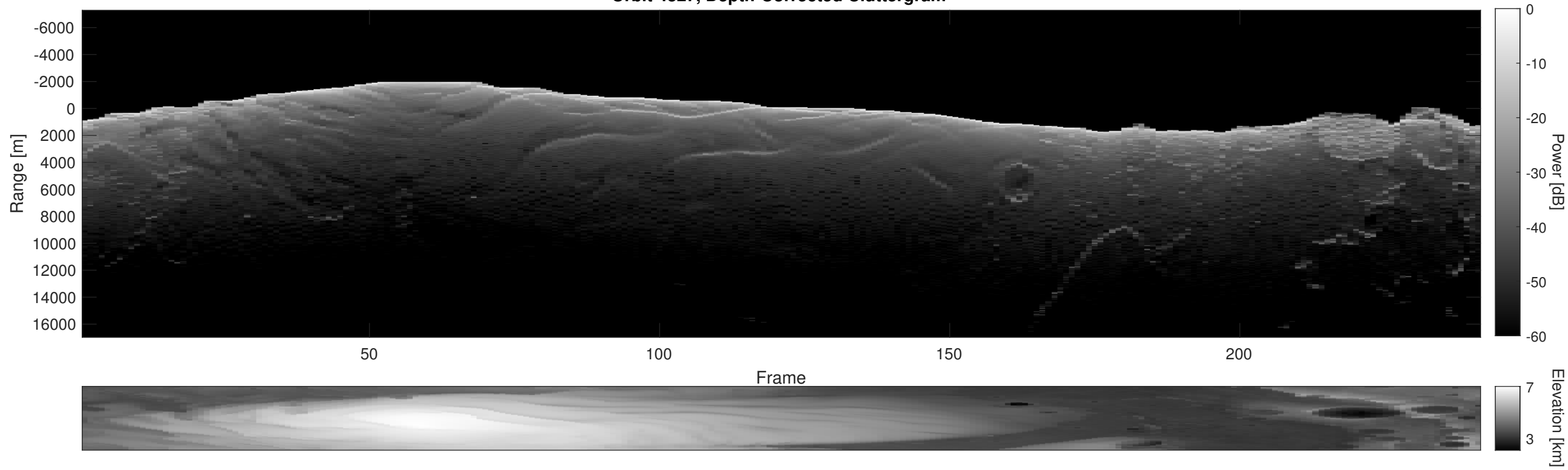
Orbit 4327, Depth-Corrected Cluttergram
