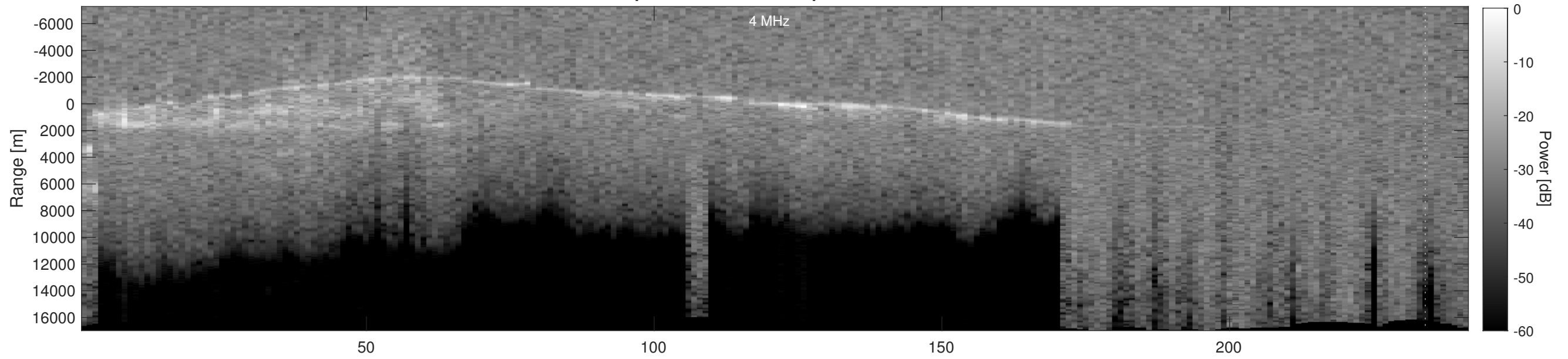
Orbit 4327, Depth-Corrected Cluttergram
