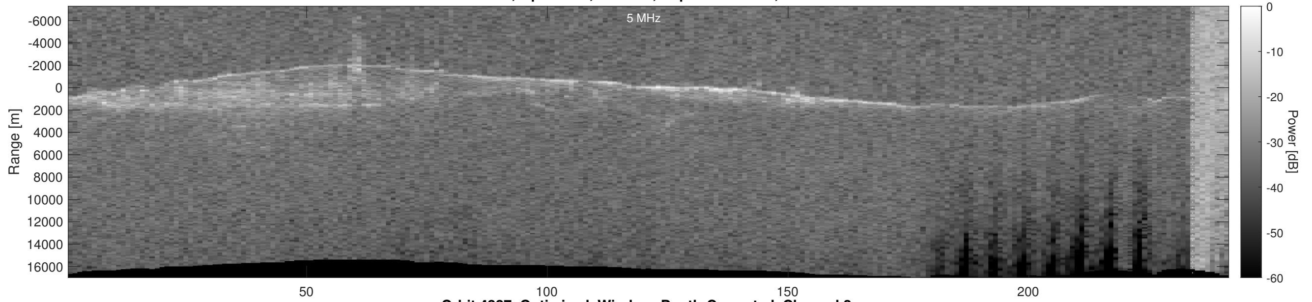
Orbit 4327, Optimized, Window, Depth-Corrected, Channel 2
