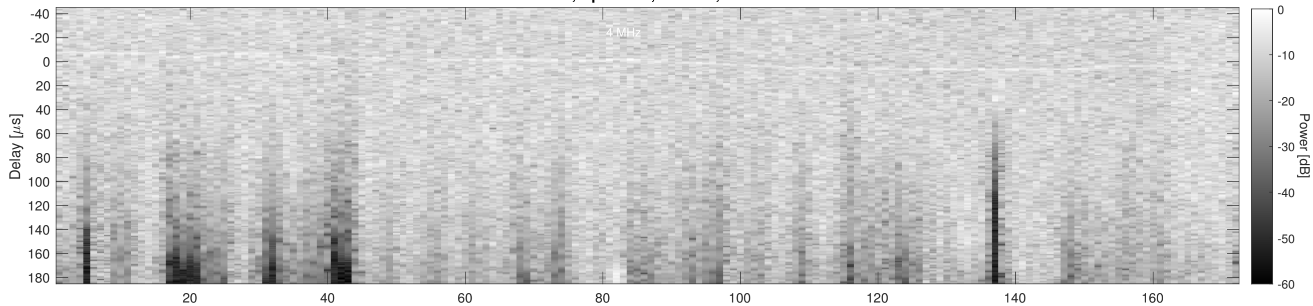
Orbit 4330, Cluttergram
