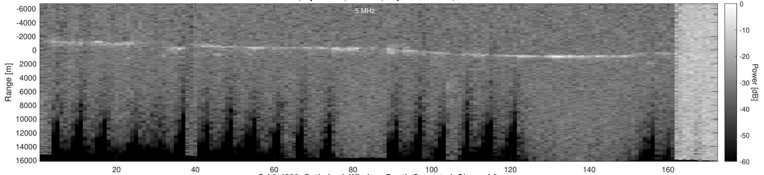
Orbit 4330, Optimized, Window, Depth-Corrected, Channel 2
