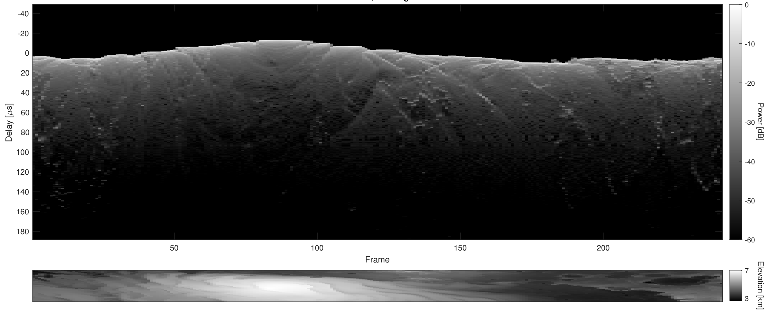
Orbit 4331, Cluttergram
