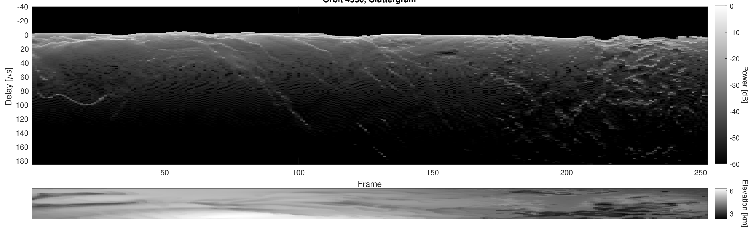
Orbit 4336, Cluttergram
