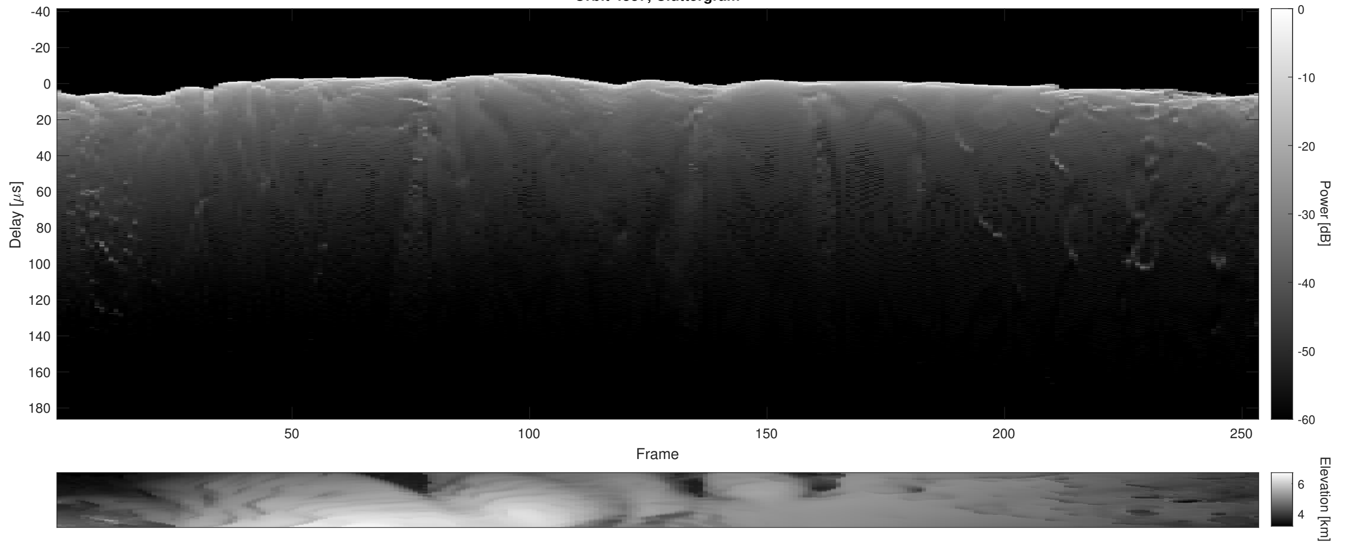
Orbit 4337, Cluttergram
