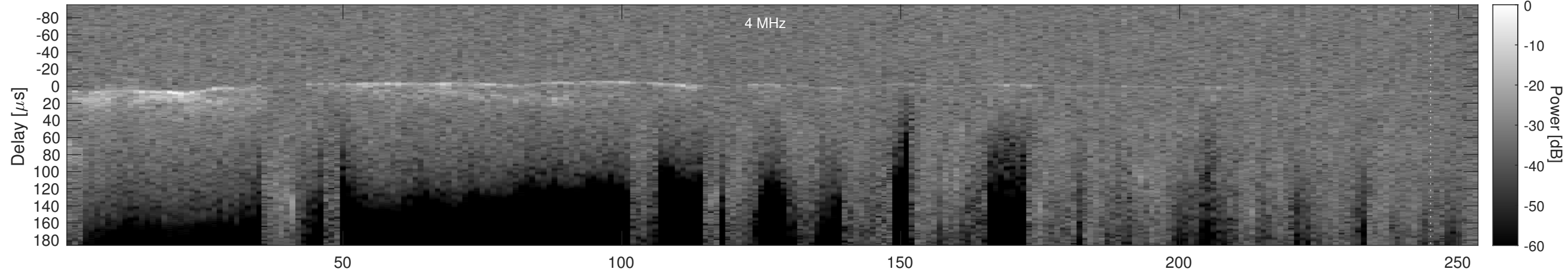
Orbit 4337, Cluttergram
