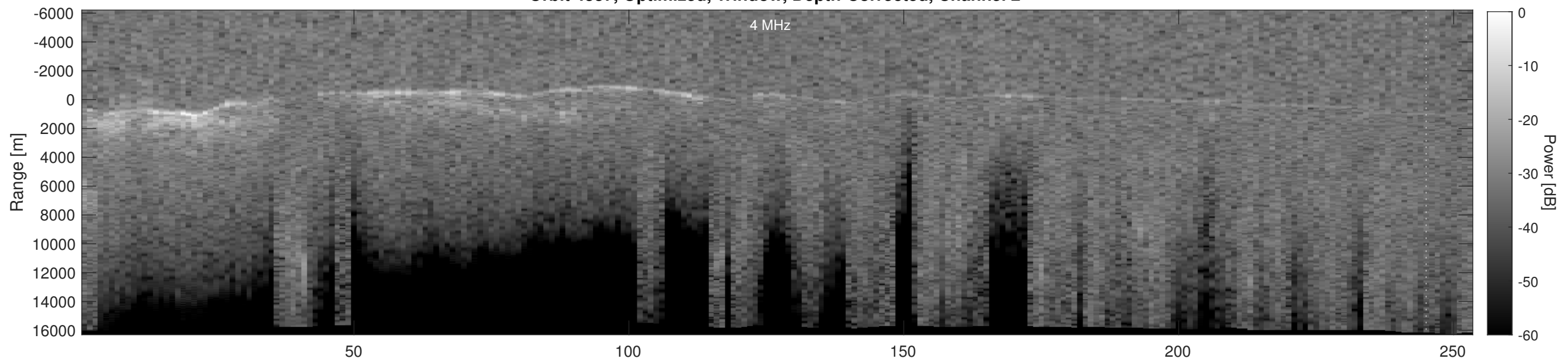
Orbit 4337, Depth-Corrected Cluttergram
