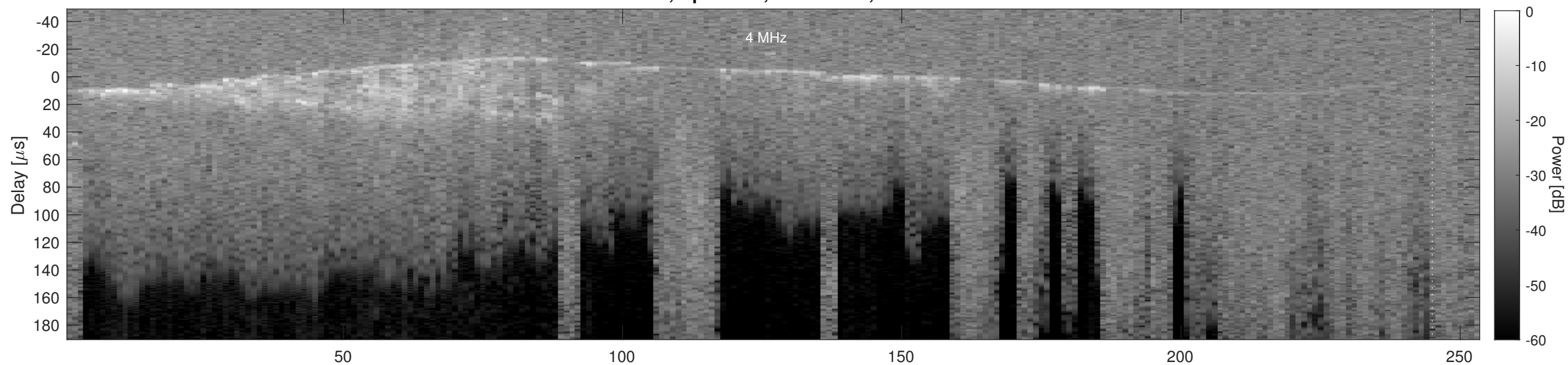
Orbit 4338, Cluttergram
