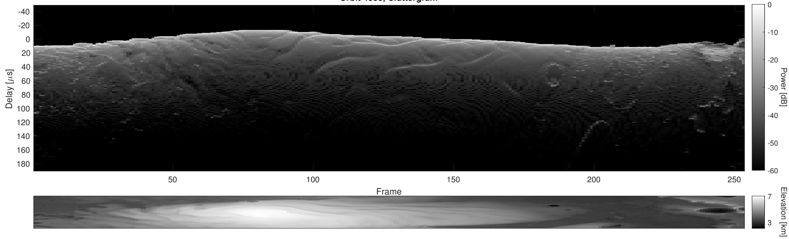
Orbit 4338, Cluttergram
