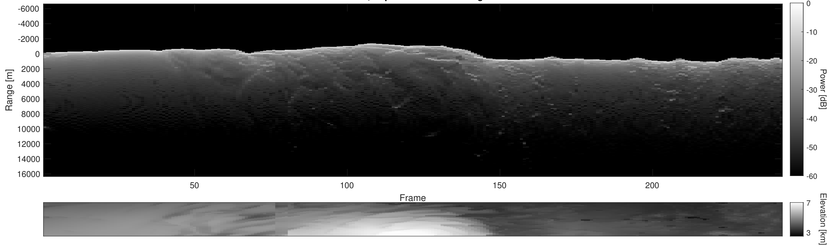
Orbit 4339, Depth-Corrected Cluttergram
