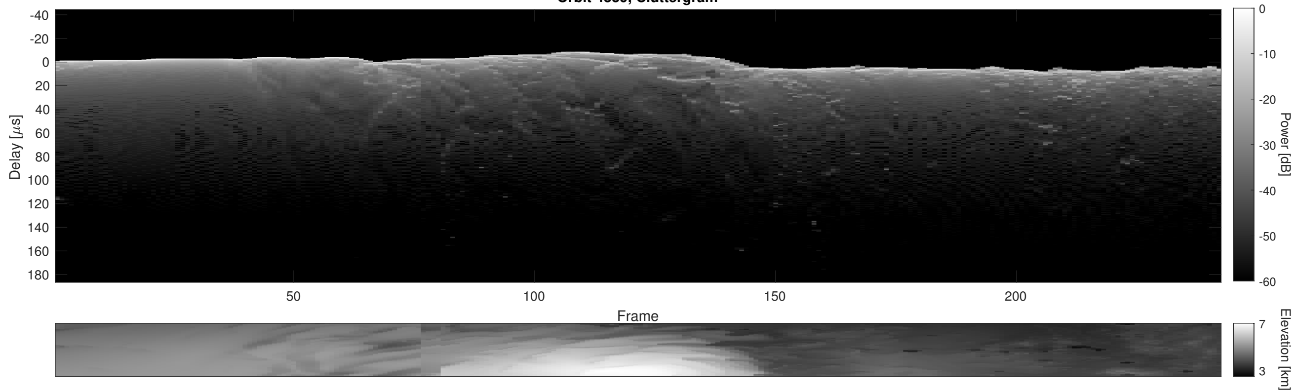
Orbit 4339, Cluttergram
