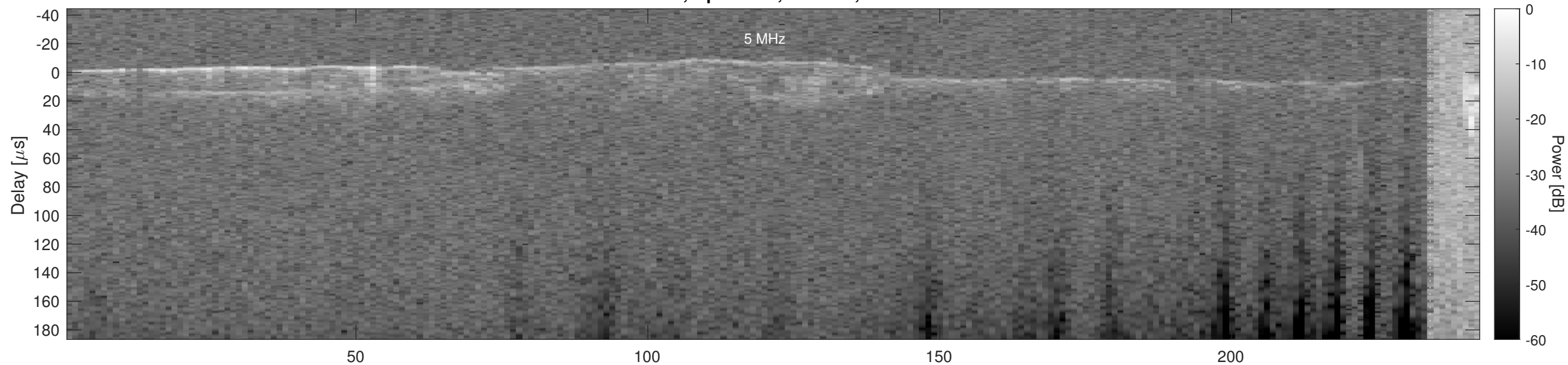
Orbit 4339, Optimized, Window, Channel 2
