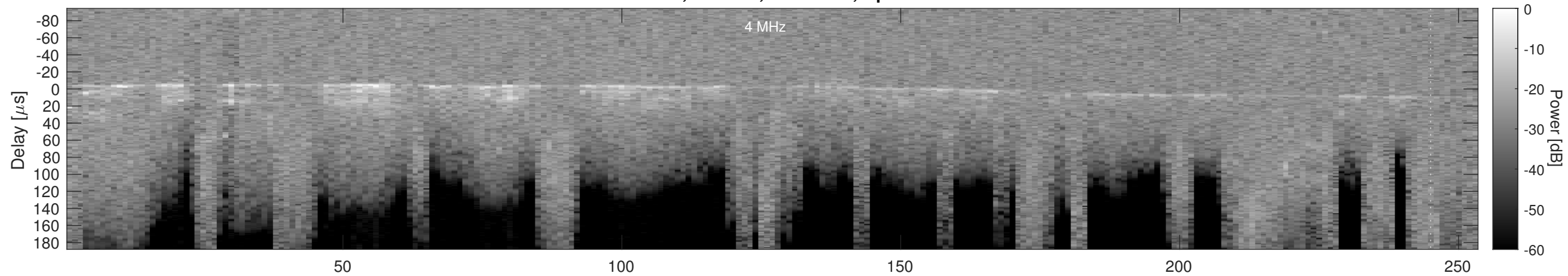
Orbit 4343, Cluttergram
