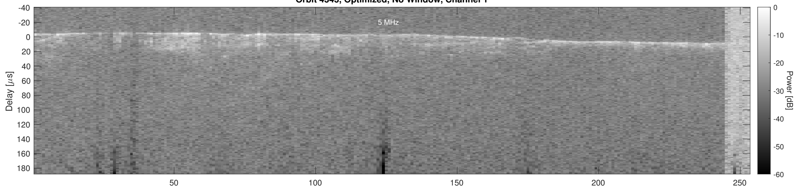
Orbit 4343, Optimized, No Window, Channel 2
