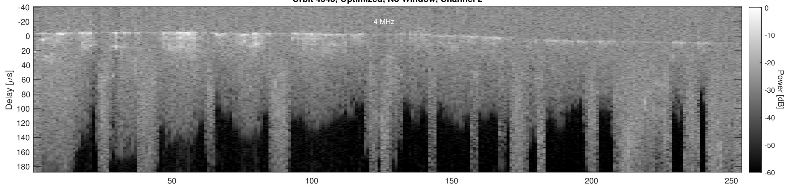
Orbit 4343, Cluttergram
