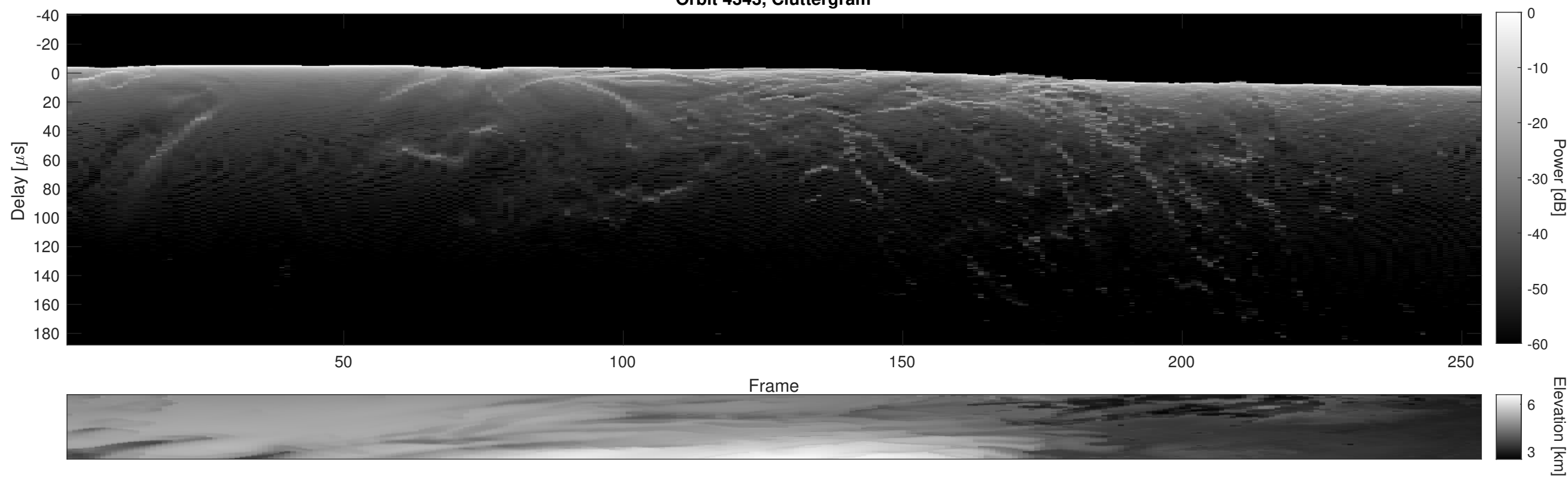
Orbit 4343, Cluttergram
