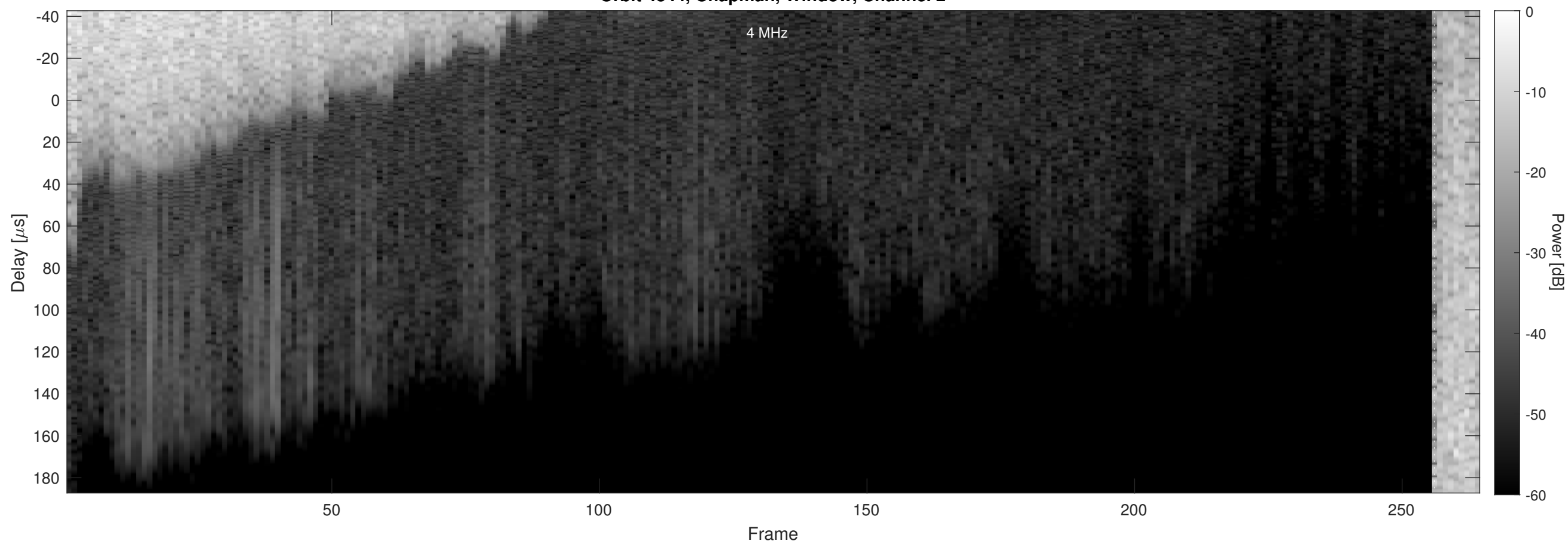
Orbit 4344, Chapman, Window, Channel 2
