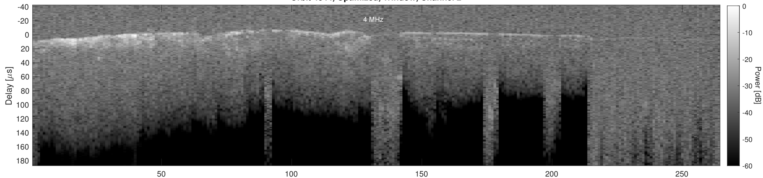
Orbit 4344, Cluttergram
