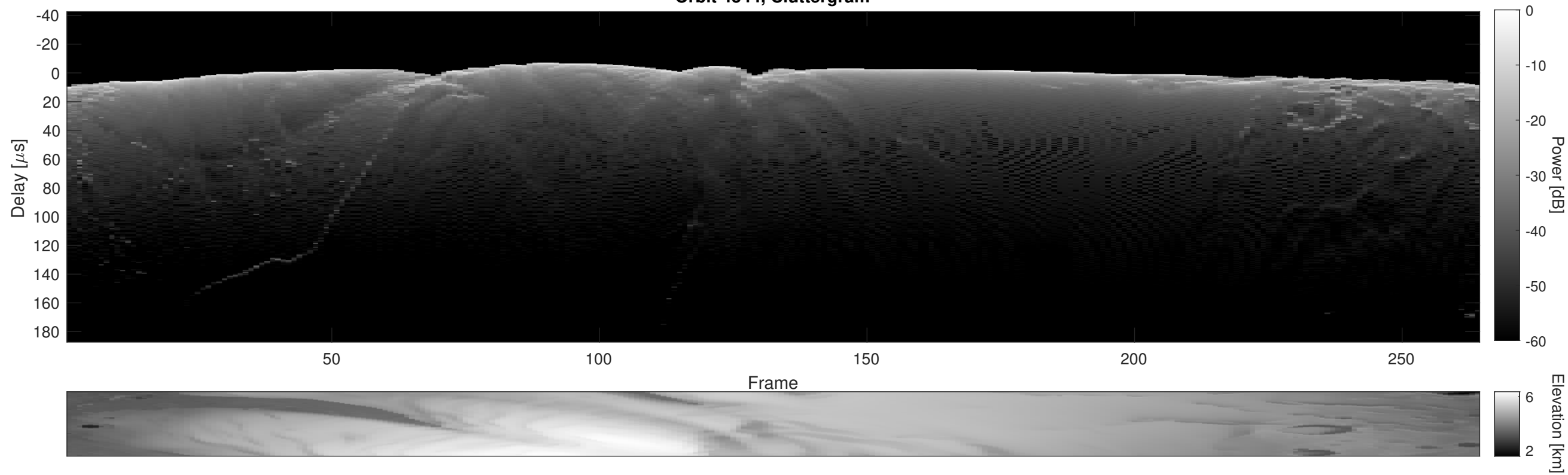
Orbit 4344, Cluttergram
