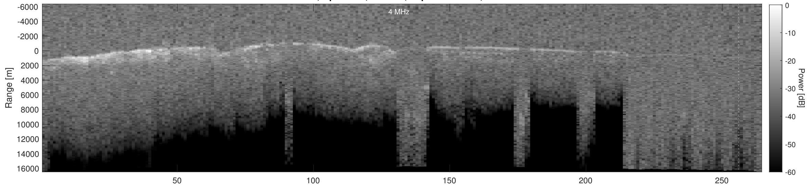
Orbit 4344, Depth-Corrected Cluttergram
