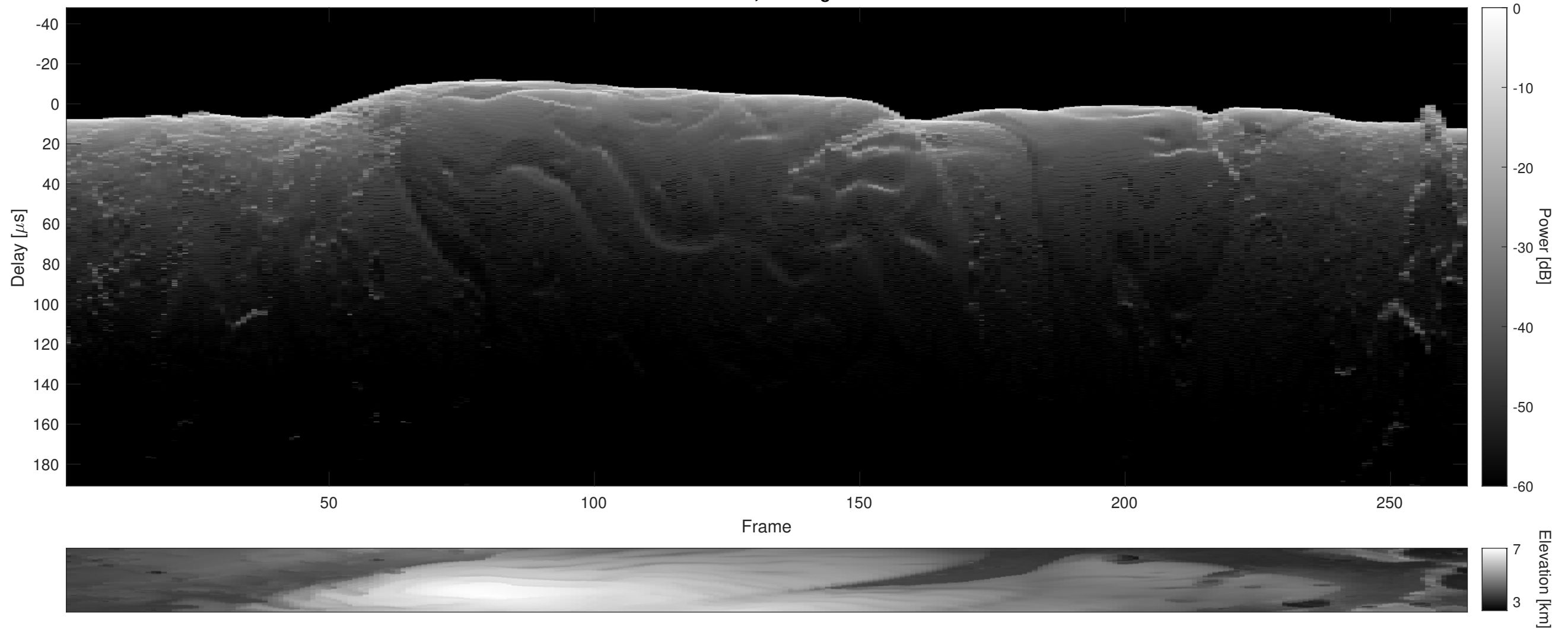
Orbit 4345, Cluttergram
