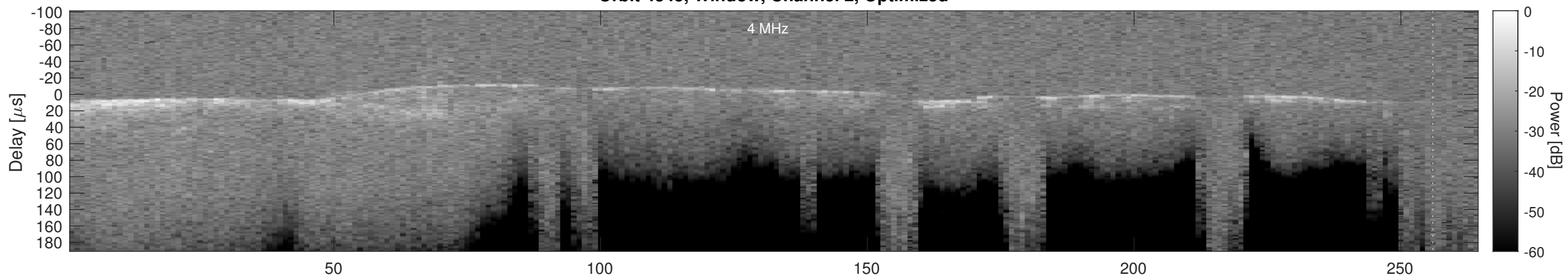
Orbit 4345, Cluttergram
