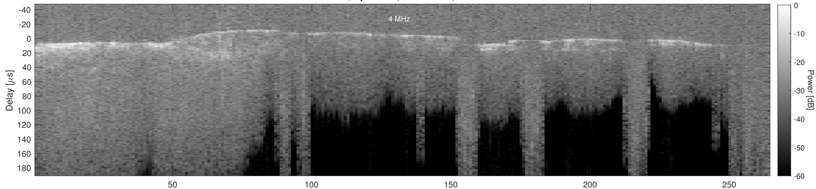
Orbit 4345, Cluttergram
