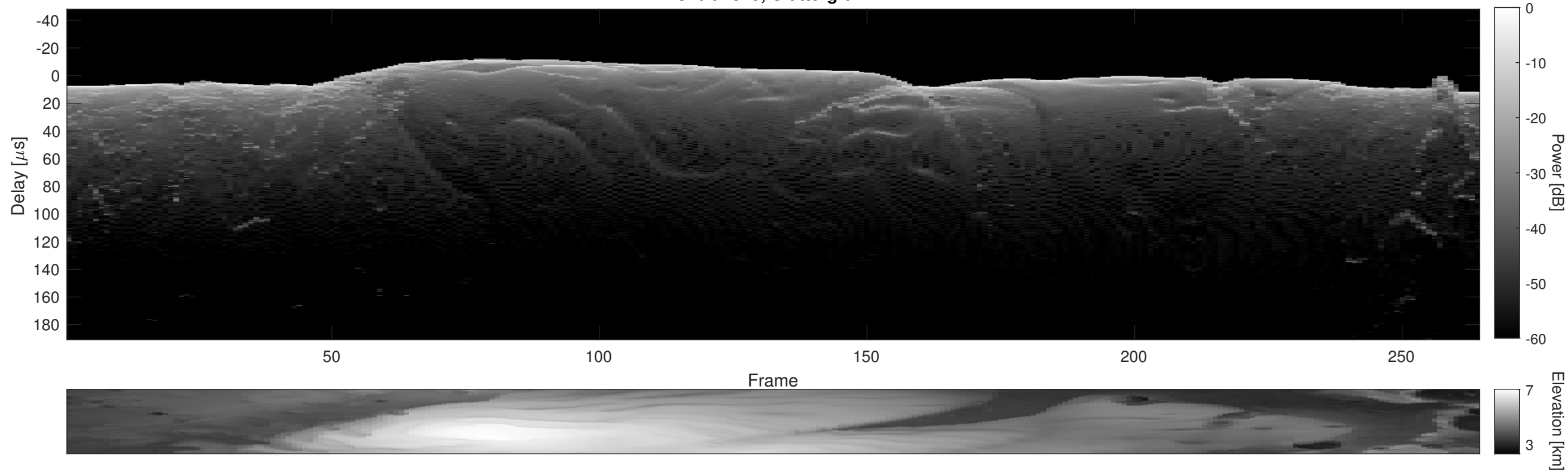
Orbit 4345, Cluttergram
