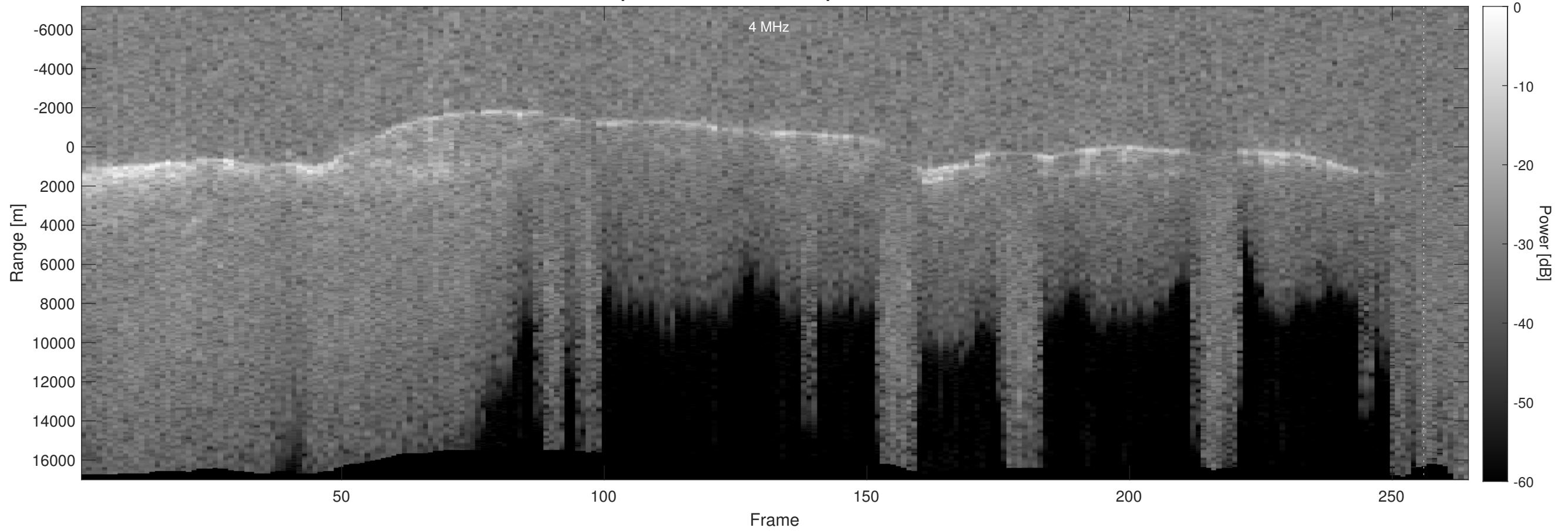
Orbit 4345, Optimized, No Window, Depth-Corrected, Channel 2
