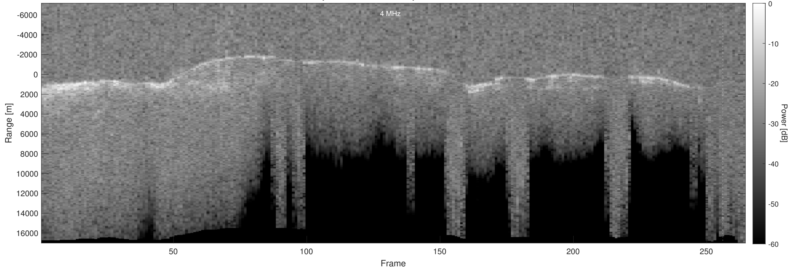
Orbit 4345, Optimized, Window, Depth-Corrected, Channel 2
