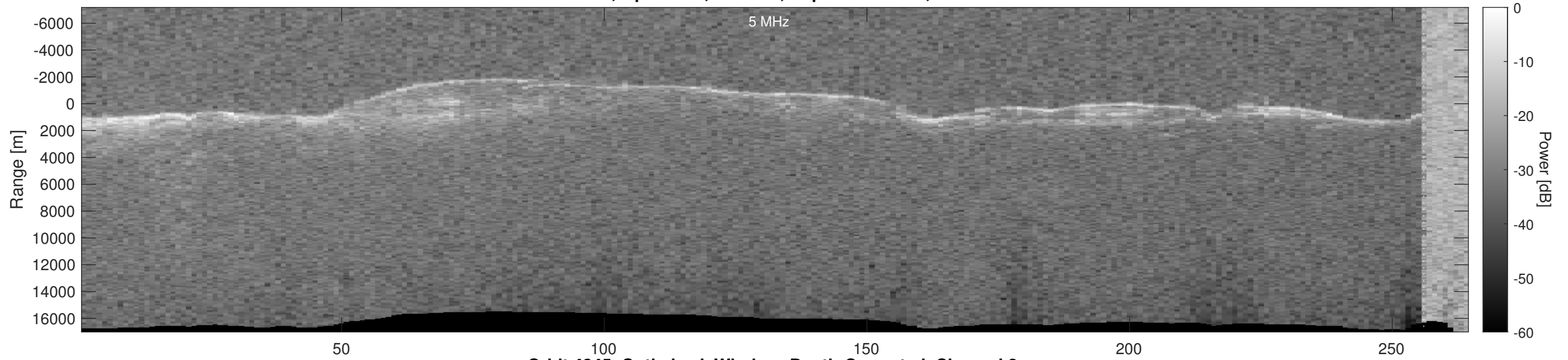
Orbit 4345, Optimized, Window, Depth-Corrected, Channel 2
