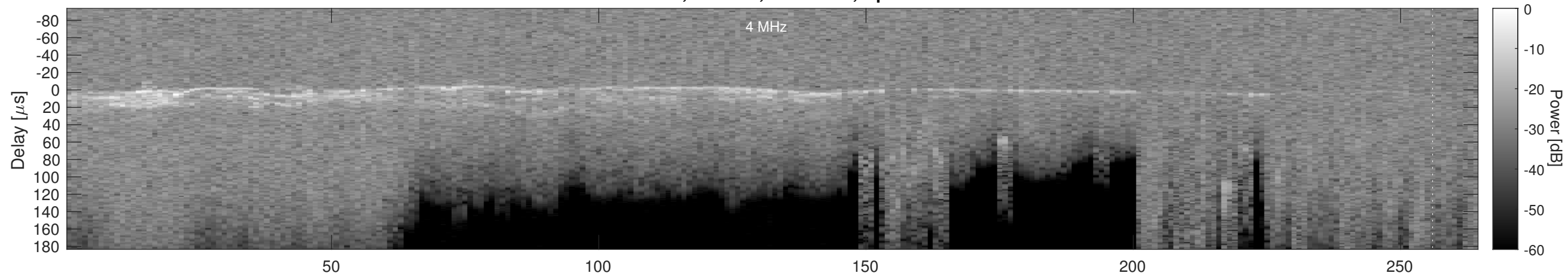
Orbit 4347, Cluttergram
