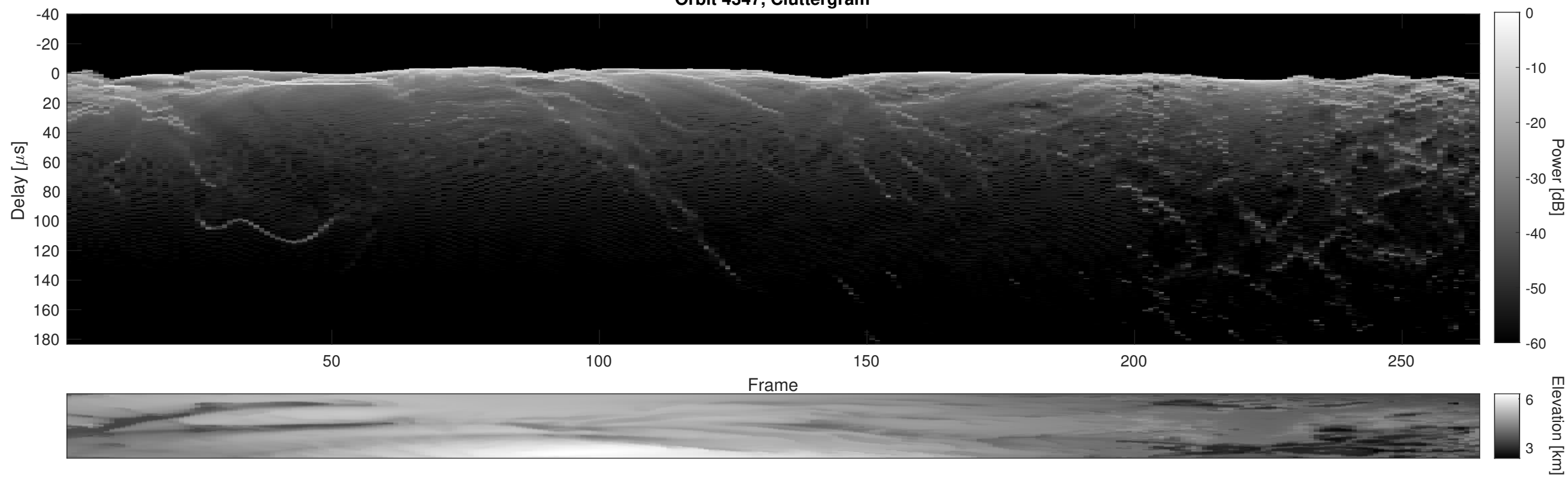
Orbit 4347, Cluttergram
