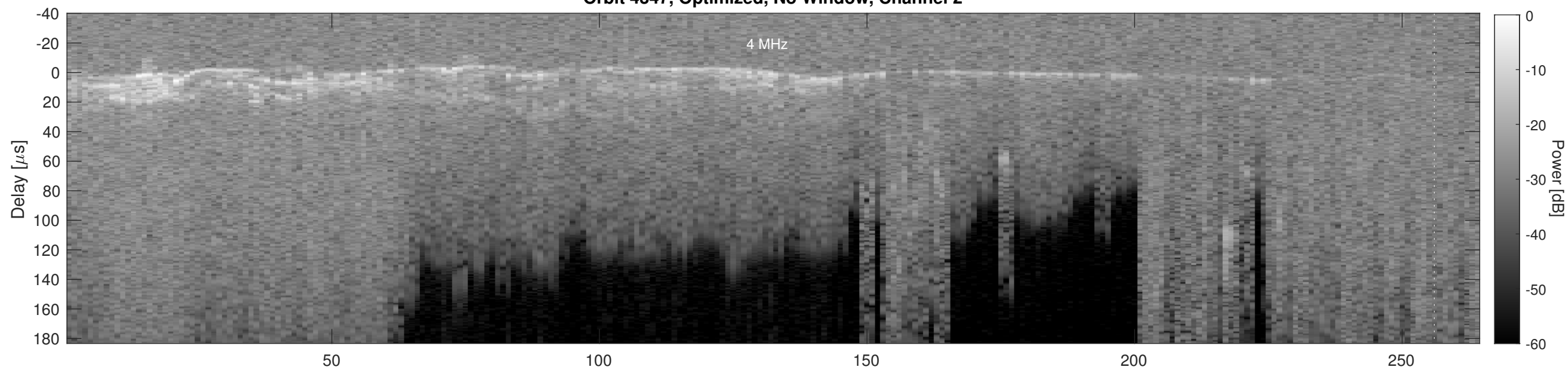
Orbit 4347, Cluttergram
