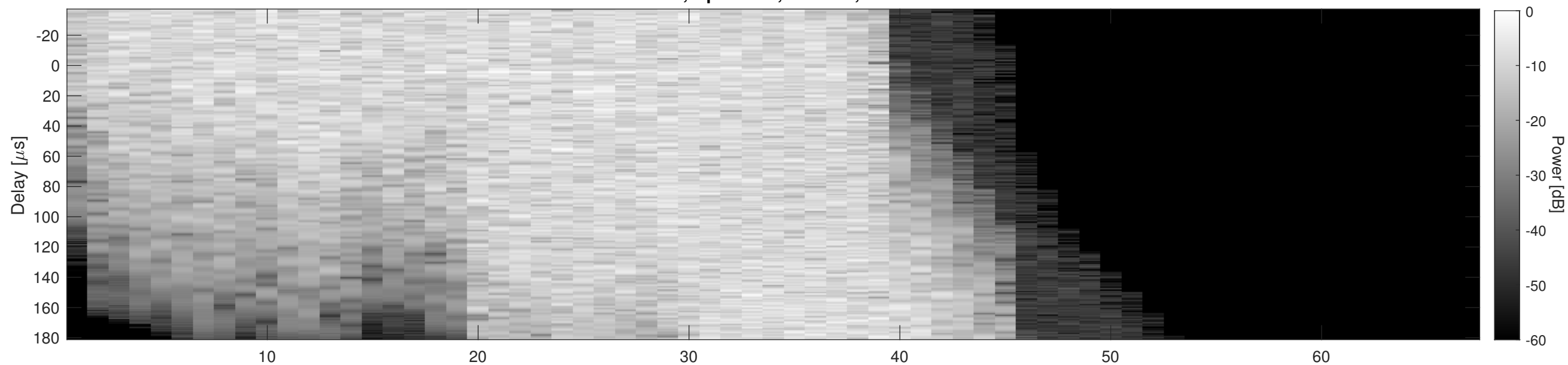
Orbit 4348, Cluttergram
