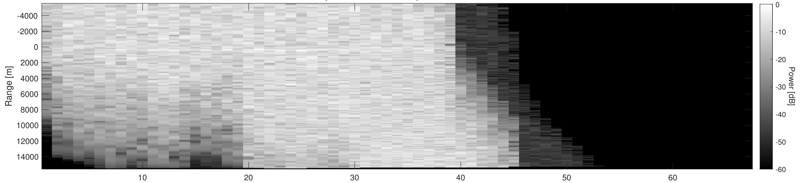
Orbit 4348, Depth-Corrected Cluttergram
