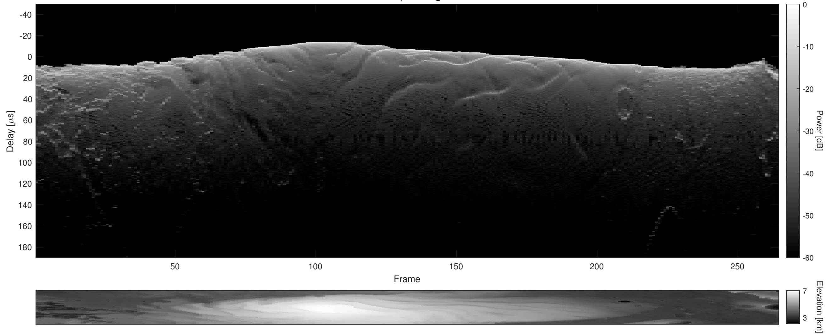
Orbit 4349, Cluttergram
