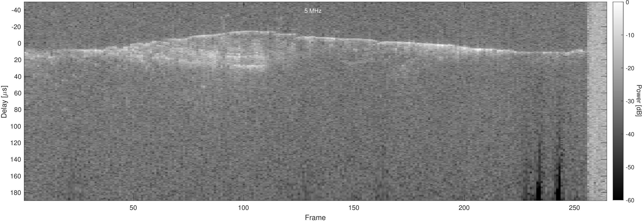
Orbit 4349, Optimized, No Window, Channel 2
